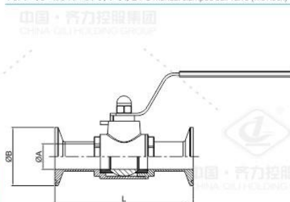
两片式手动快装球阀(带锁) 2-PC manual clamped ball valve (with lock)
