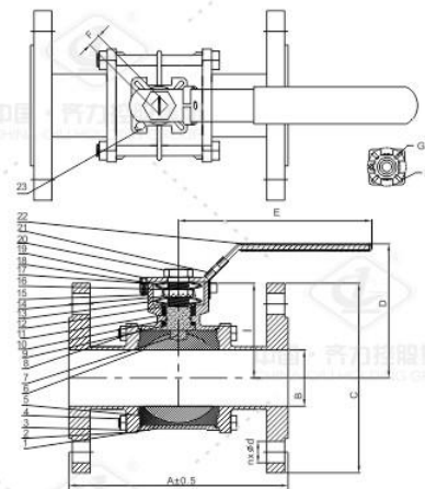
1/2"-6" Encapsulated and ISO mounting pad. Flange connection size please refer to the standard ISO5211
