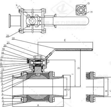
DN10-DN100 Encapsulated and ISO mounting pad. Flange connection size please refer to the standard ISO5211
