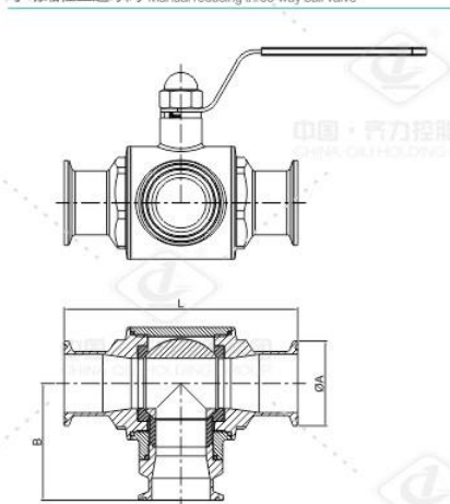
手动缩径三通球阀 Manual reducing three-way ball valve
