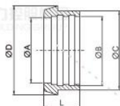
DIN-14 WELDING LINER
