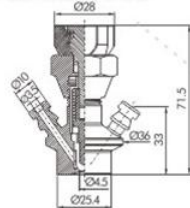
焊接式无菌取样阀 Welded Aseptic Sampling Valve
