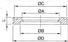
承插法兰 ISO Bored Flange
