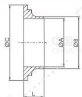
SMS-14GL LONG WELDING LINER
