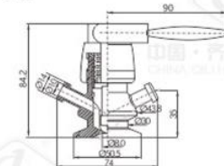
卡箍式无菌取样阀 Clamped Aseptic Sampling Valve
