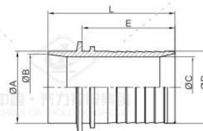
焊接扣压接头 Welded hose adapter
