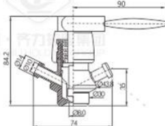
焊接式无菌取样阀 Welded Aseptic Sampling Valve
