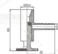
焊接式取样阀 Welded Sampling Valve
