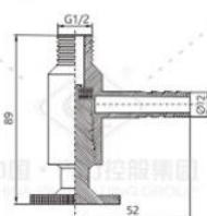
螺纹式取样阀 Thread Sampling Valve
