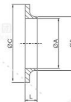
SMS-14S SHORT WELDING LINER
