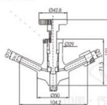
焊接式无菌取样阀 Welded Aseptic Sampling Valve
