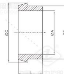
DIN-14 WELDING LINER
