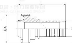
RJT公头扣压接头 RJT Male hose adapter
