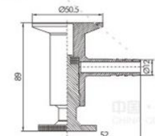
卡箍式取样阀 Clamped Sampling Valve
