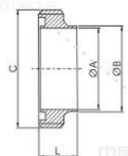
SMS-15GL LONG WELDING MALE
