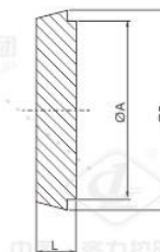
DIN-15 DA/DB WELDING LINER
