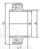
螺纹接头 Threaded female
