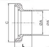
DIN-151IMPERIAL WELDING MALE
