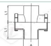
直通焊接式视镜 Welding sight glass 3A/SMS/ISO/IDF No.QL-082 SIZE L1 B A 1" 130 25.4 79 1 1/2" 128 38.1 85 2" 133 50.8 100 2 1/2" 131 63.5 115 3" 134 76.2 127 4" 135 101.6 156 无电缆灯视镜 Cable-free lamp sight glass DIN No.QL-086 SIZE A L1 L2 DN65 70 121.5 31 DN80 85 123.5 33 DN100 104 126.5 37 DN125 129 127.5 38 DN150 154 133.5 45 卡箍式直通视镜 Clamp sight glass 3A/SMS/ISO/IDF No.QL-083 SIZE L1 K1 A 1" 153 50.5 79 1 1/2" 151 50.5 85 2" 155 64 100 2 1/2" 153 77.5 115 3" 156 91 127 4" 165 119 156 带灯视镜 Lamp sight glass DIN No.QL-087 SIZE L1 B A DN80 90 87 126 DN100 100 106 146 DN125 90 132 178 DN150 96 157 208 179 Professional Manufacturer FDA TS CE CHINA QILI GROUP 180
