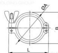
KF-卡箍-铝制 KF-Clamp-Aluminum
