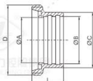
DIN-15R EXPANDING WELDING MALE
