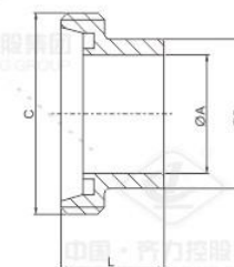
DIN-14 DA/DB WELDING LINER
