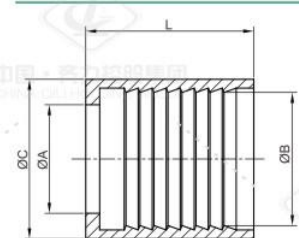
软管接头套筒 Hose clamp
